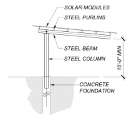
3 ARRAY SECTION Scale: 1/8" = 1'-0" (FOR 24X36 SHEETS)
