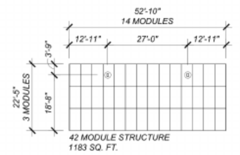
2 ARRAY LAYOUT Scale: 1/16" = 1'-0" (FOR 24X36 SHEETS)
